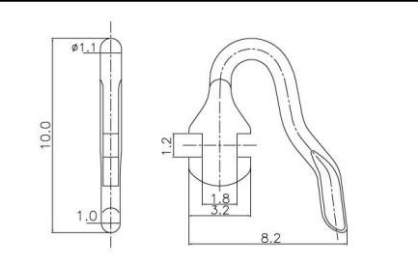
TPA-01NS Material: Nickel silver
